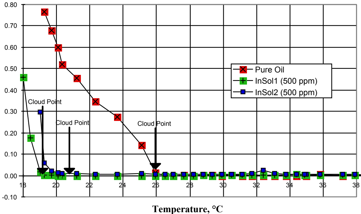
InSol Performance as Wax Inhibitor Wax Cloud Point Suppression East European Stock Tank Oil
